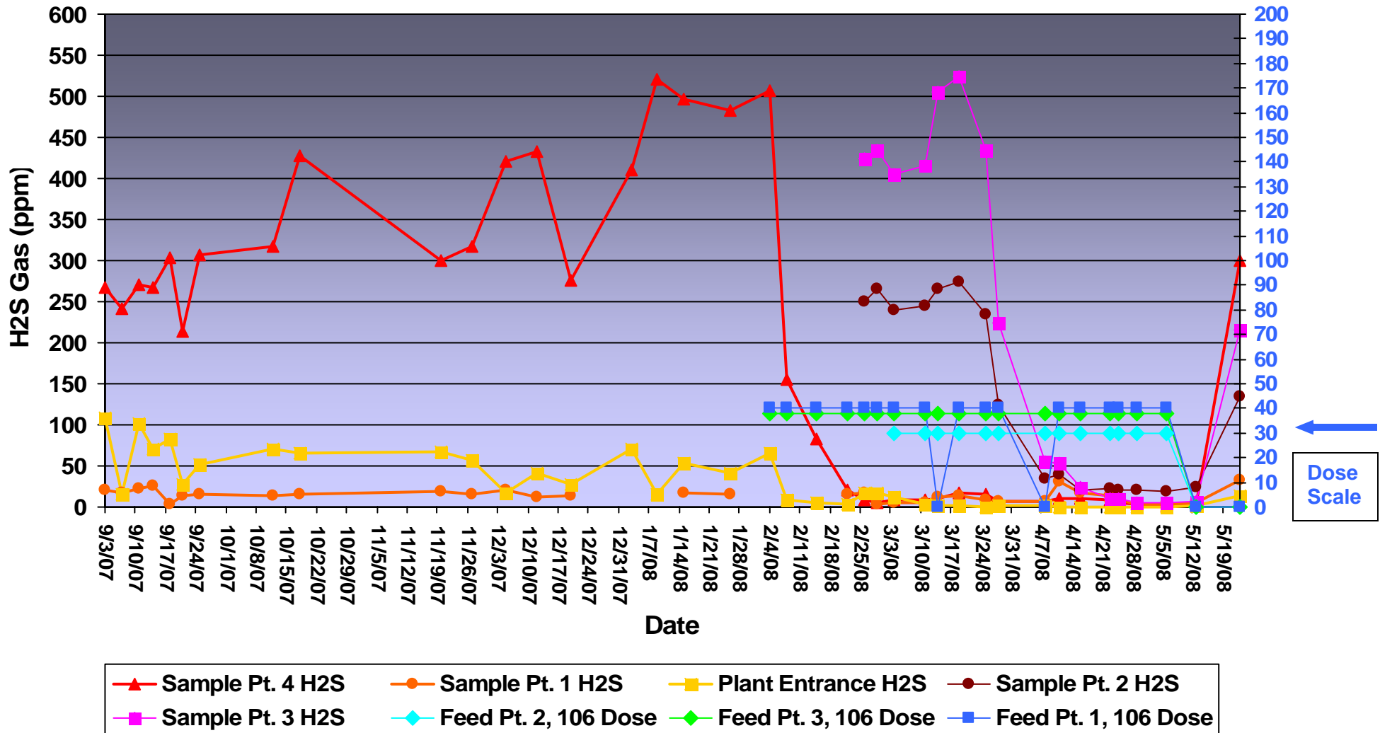
Graph 1 - Municipal Wastewater System RoeTech 106 - H2S Gas Removal
